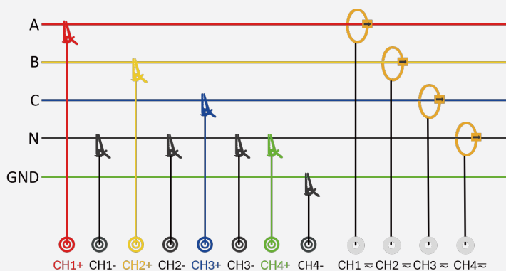
3P4W WYE Connection
